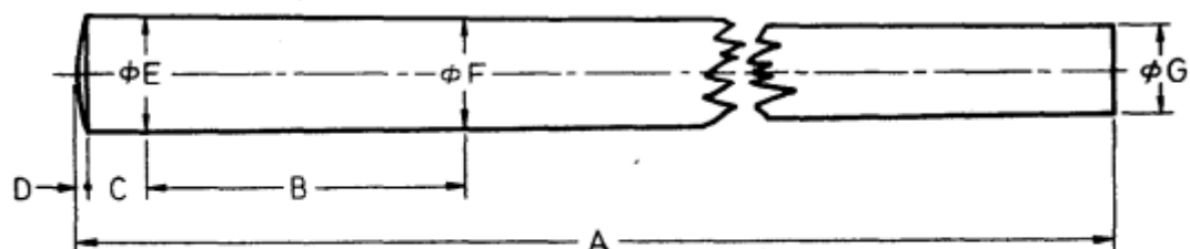
Fig. 1 Handle for Adze 1.5 kg (Type A)
